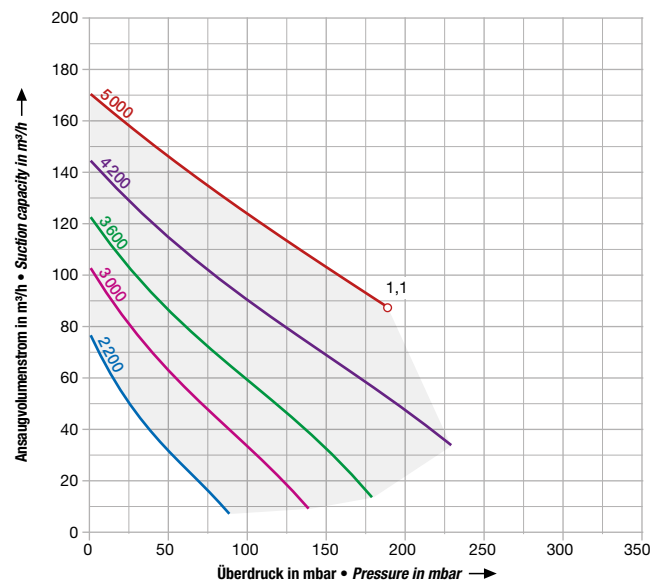
2BH1 430
