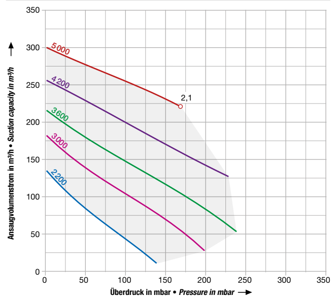
2BH1 530
