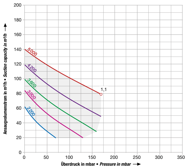
2BH1 400
