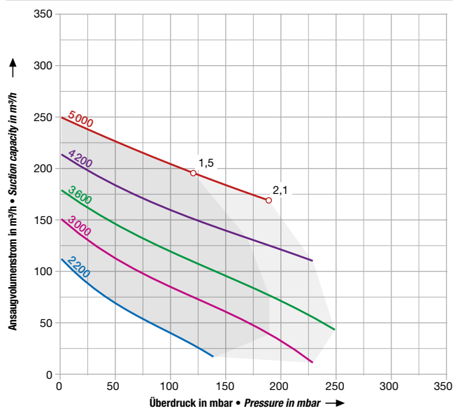
2BH1 500
