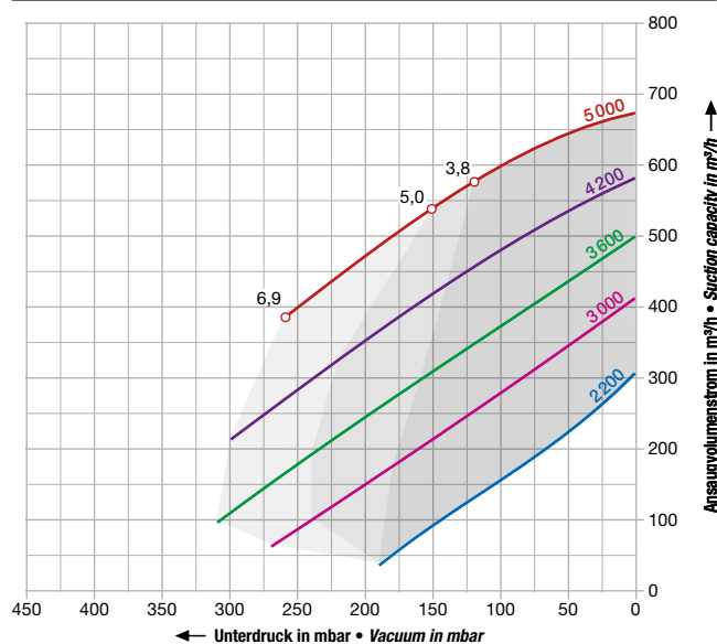
2BH1 800
