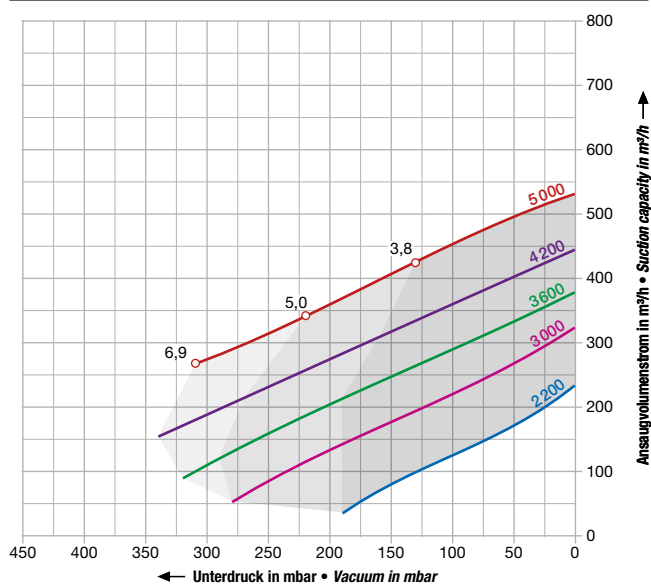
2BH1 640
